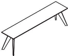
Woody Bank / Woody Bank gepolstert Woody Bank / Woody Bank padded 6 Breiten / 6 widths: 100, 120, 140, 160, 180, 200 cm Tiefe / depth: 30 cm Höhe / height: 47 cm Höhe gepolstert / height padded: 52 cm
